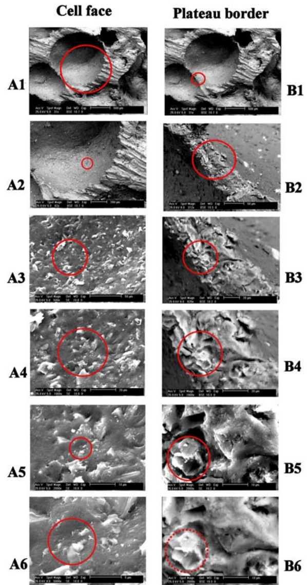
Al-7%Si-3%SiC-1%TiH 2
