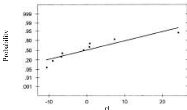
Average: 0.000001 Std Dev: 10.7610 N of data: 9 Anderson-Darling Normality Test A-Squared: 0.566 p-value: 0.101
