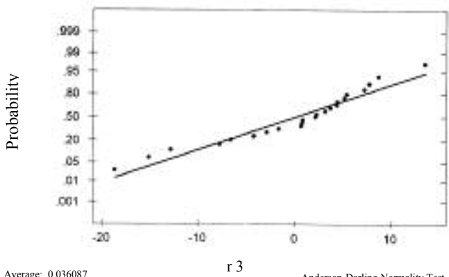
Average: 0.036087 Std Dev: 7.91234 N of data: 23 Anderson-Darling Normality Test A-Squared: 0.622 p-value: 0.093
