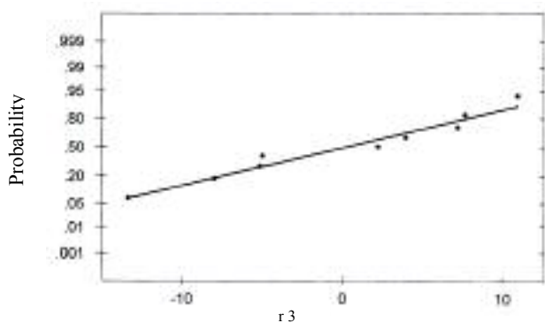
Average: 0.0811111 Std Dev: 8.2433 N of data: 9 Anderson-Darling Normality Test A-Squared: 0.276 p-value: 0.564
