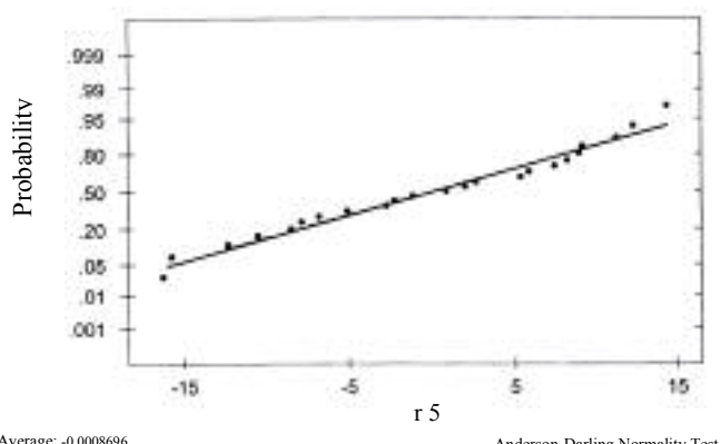
Average: -0.0008696 Std Dev: 9.14766 N of data: 23 Anderson-Darling Normality Test A-Squared: 0.280 p-value: 0.613
